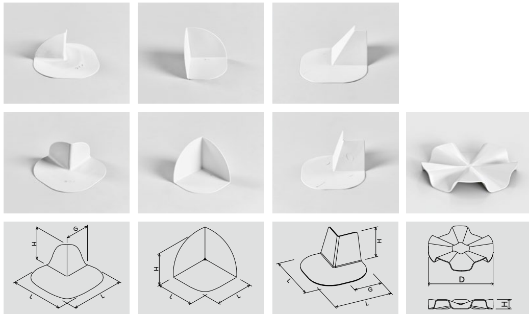
270° External Corner
